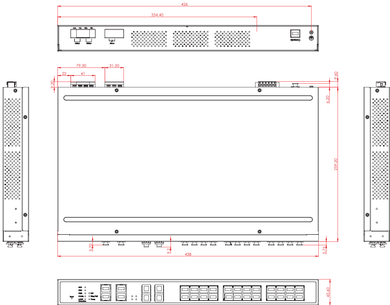
Figure 1-5. EKI-7428G-4CI Dimensions
