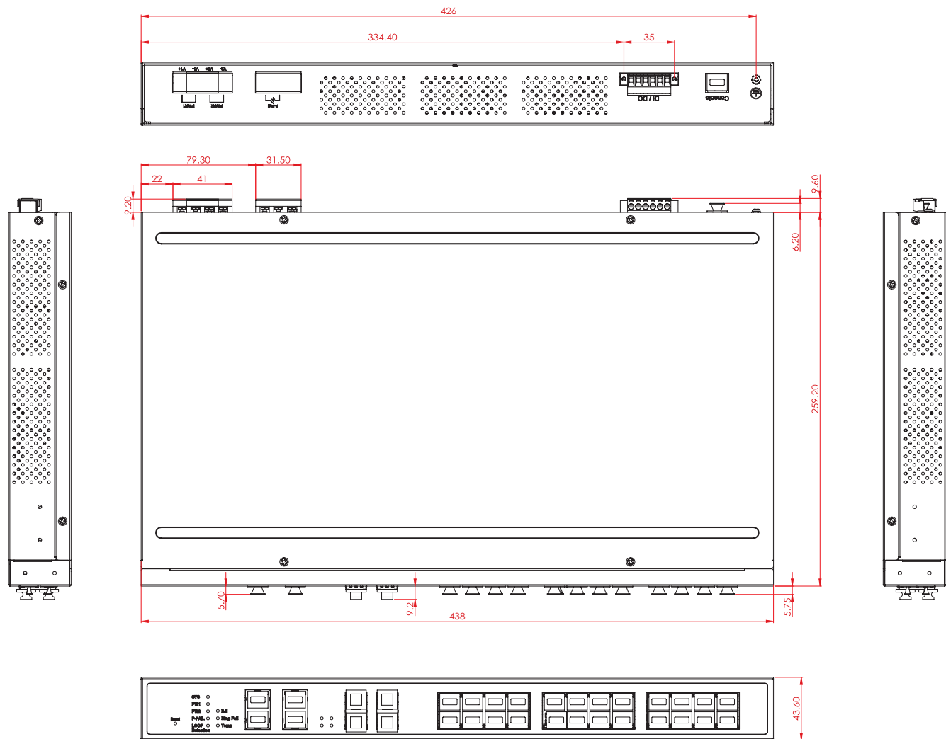
Figure 1-4. EKI-7428G-4CPI Dimensions
