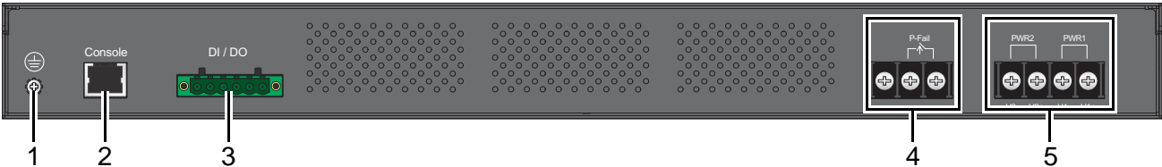
Figure 1-3. Rear View
