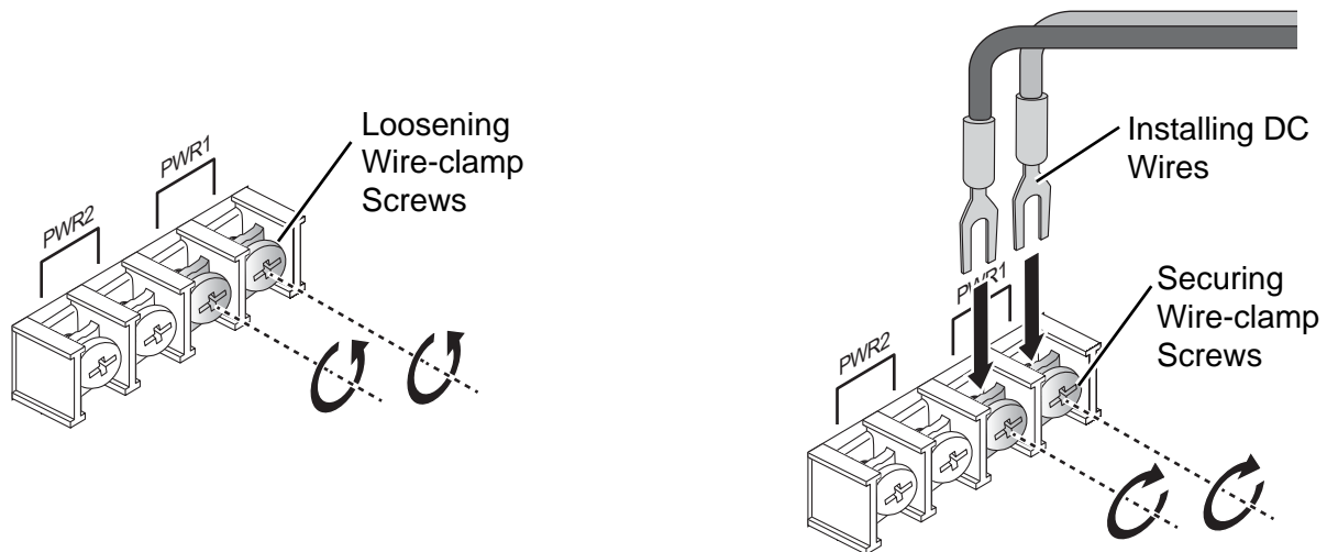
Figure 2-16. Installing DC Wires in a Terminal Block
