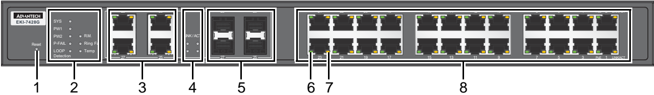
Figure 1-1. Front View
